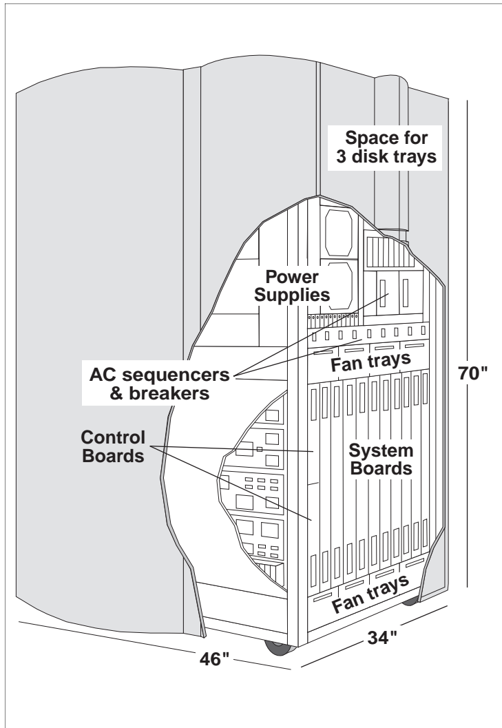
Figure 4. Starfire cabinet
