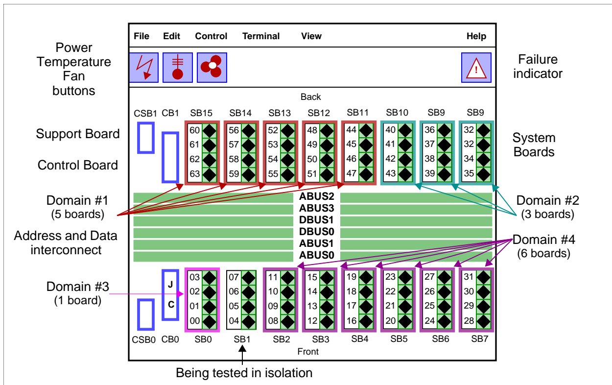
Figure 7. SSP hostview main screen
