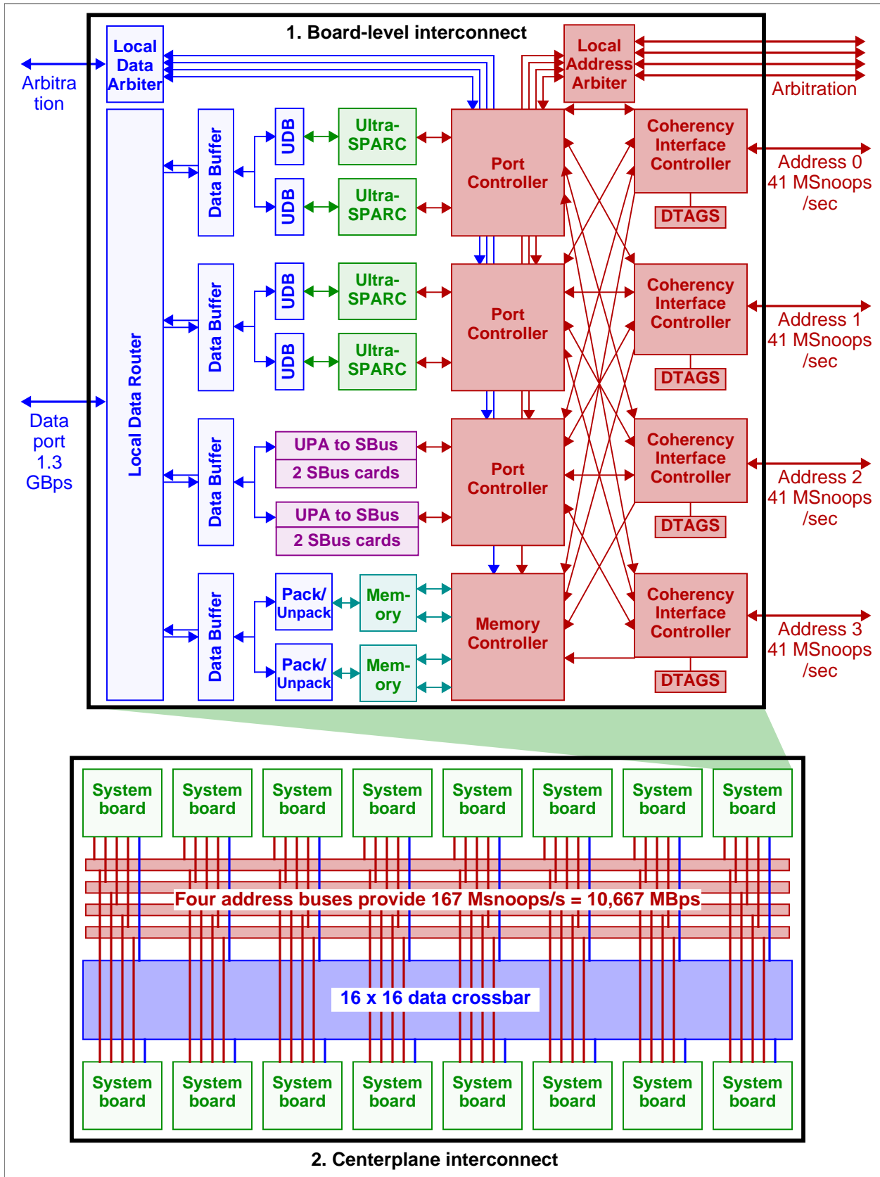
Figure 3. Starfire interconnect
